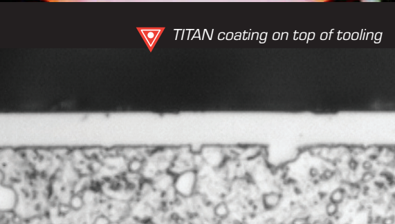
TITAN core pin applications
