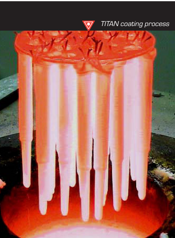
TITAN coating on top of tooling
